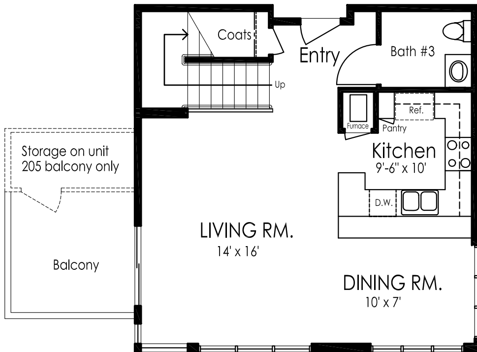
First Floor Plan Plan T1 is shown
